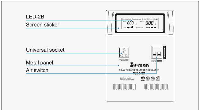
FRONT PANEL
