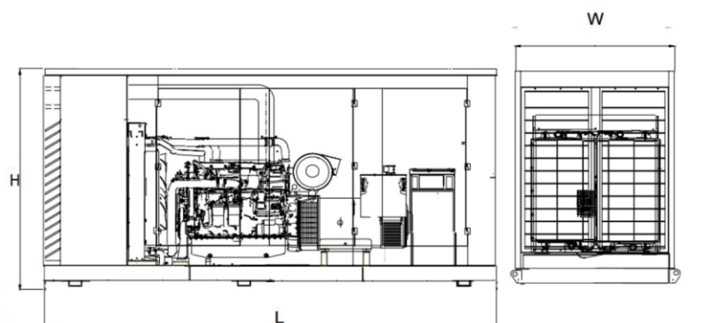
Generator with Soundproof Canopy
